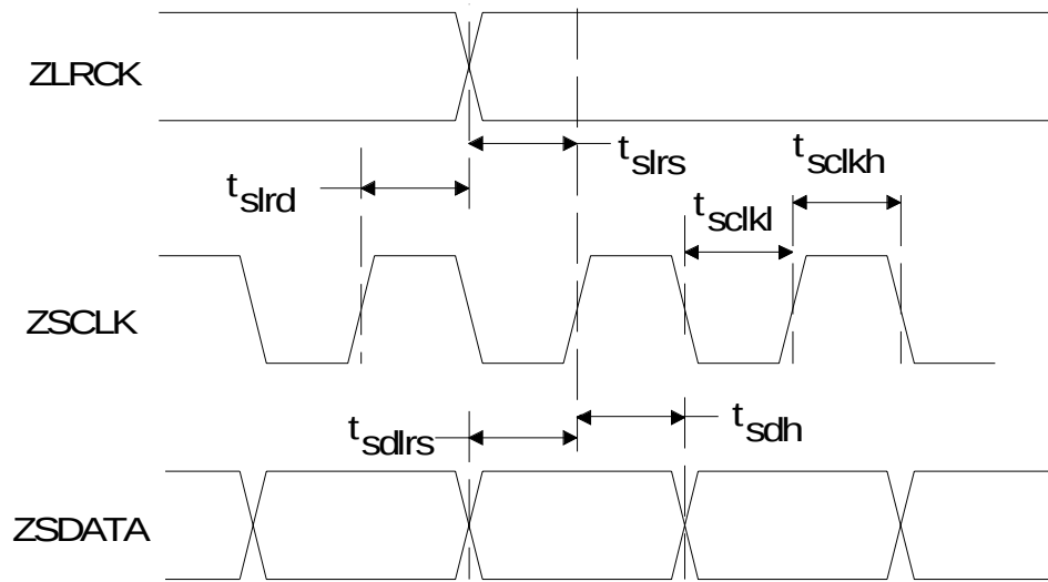
ZV-Port Input Timing
