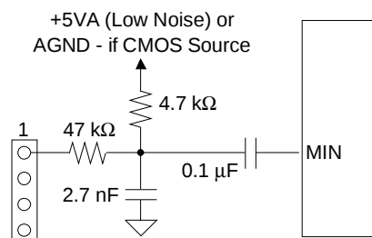
Figure 22. Mono Input
