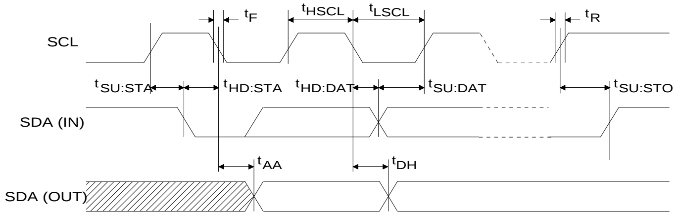
E²PROM 2-Wire Interface Timing
