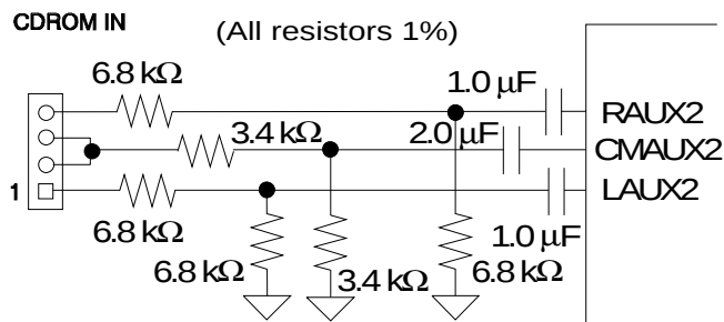
Figure 20. Differential CDROM In
