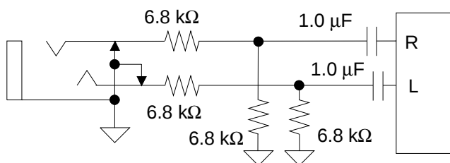
Figure 19. Line Inputs
